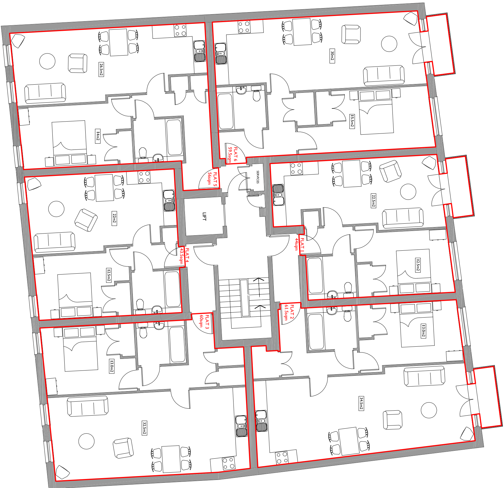
FIRST FLOOR PLAN SCALE 1:100 (@A3)
